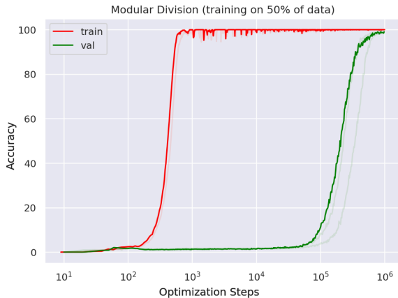
Рис. 16: Training transformer with 2 layers, width 128, and 4 attention heads, with a total of about 4 \cdot 10^5 non-embedding parameters. Reproduction of experiments ( \sim half an hour) is available here
